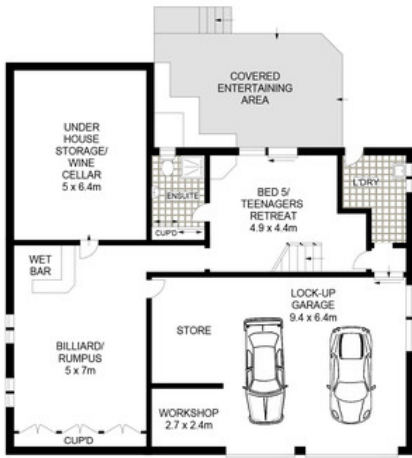
LOWER LEVEL
