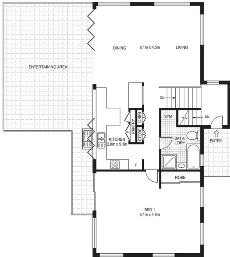
UPPER LEVEL
